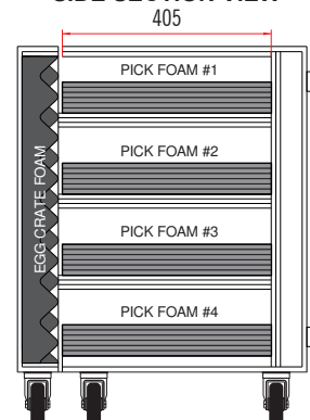
SIDE SECTION VIEW
